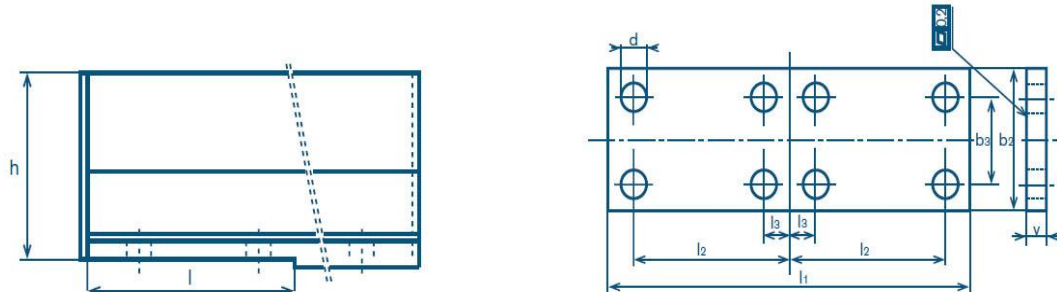
Standard fishplate.
